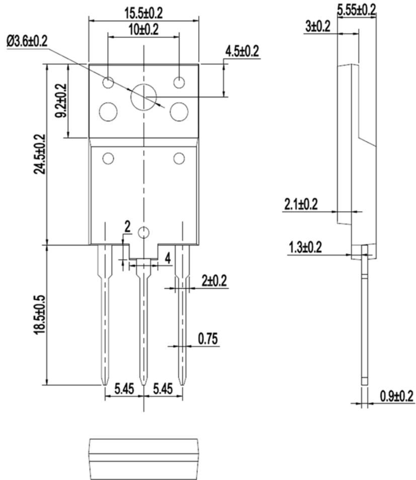
Dimensions in (mm) Figure 11. Package Outline
