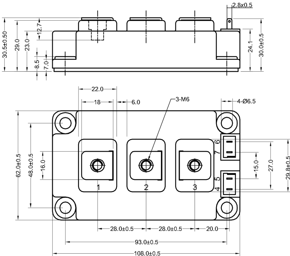
Figure 14. Package Outline
